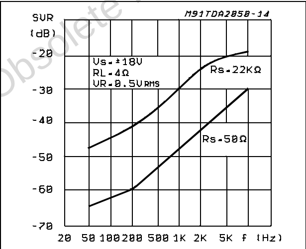
Figure 15. Supply voltage rejection vs. frequency
