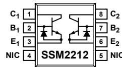
Figure 1. 8-Lead SOIC_N
