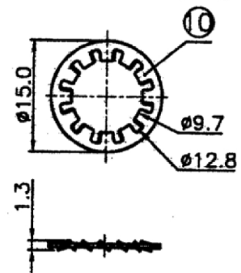
WASHER 1PC t=0.5
