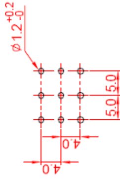
P.C.B. MOUNTING HOLE DETAIL
