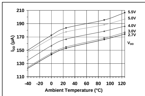
FIGURE 2-11: MCP4921 I_{DD} vs. Ambient Temperature and V_{DD} .
