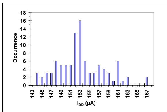
FIGURE 2-12: MCP4921 I_{DD} Histogram ( V_{DD} = 2.7\text{V} ).
