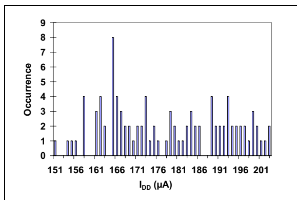
FIGURE 2-13: MCP4921 I_{DD} Histogram ( V_{DD} = 5.0\text{V} ).
