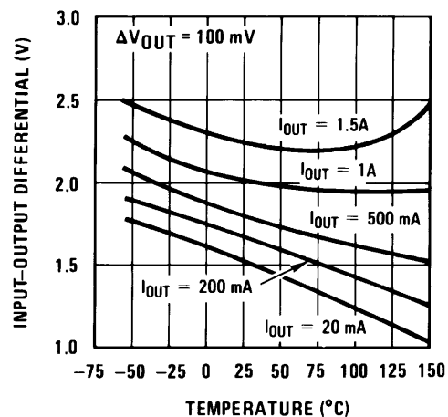
Dropout Voltage
