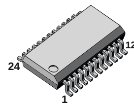
SSOP24 , 150mil, 0.635 mm
