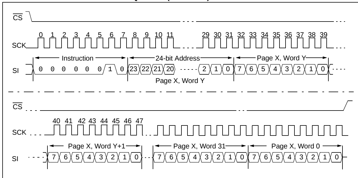
FIGURE 2-4: PAGE WRITE SEQUENCE (SPI MODE)
